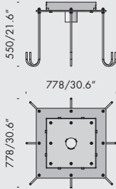
tirafondo incassato fixing in ground
