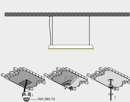
cassaforma laterizio scomparsa totale · total recessed brick housing
