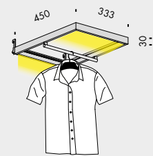
men sole 450x333/02
